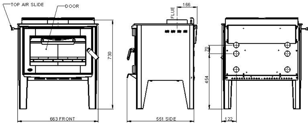
FIG. C: HEATER DIMENSIONS & WATER BOOSTER POSITION – MONTE WOODBURNER (not to scale)
